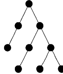
Fig. 1. Tree search of the sphere decoding algorithm.
