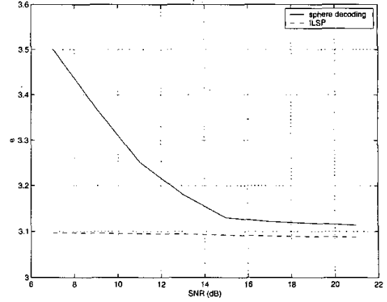
Fig. 3. Expected complexity exponent, n = 4 , T = 20 .
